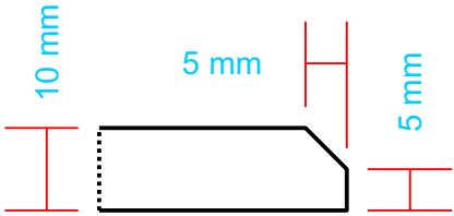
Side Profile of glass Bevel for the Top piece
